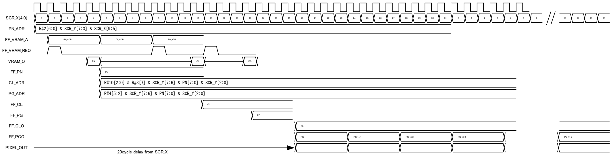
TH9958 GRAPHIC2/GRAPHIC3 timing chart
